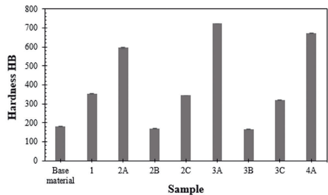
Figure 3. Graphical behavior of hardness values
