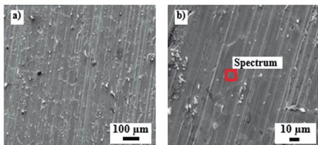
Figure 4. Micrographics of sample 3A a) 200X, and b) 1000X
