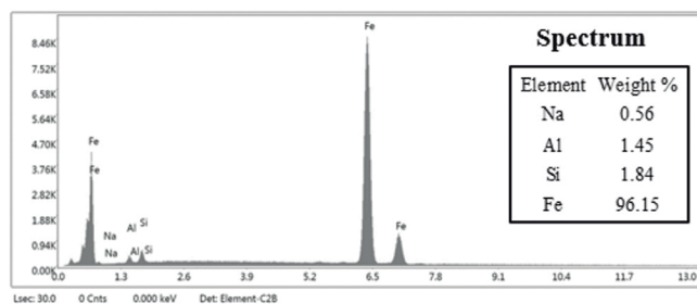
Figure 5. EDS of sample 3A
