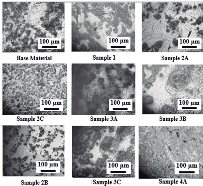
Figure 2. Metallography of the different specimens
